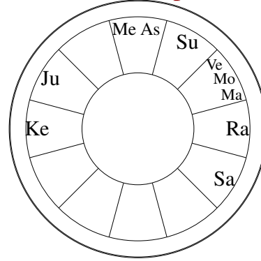
Cuspal Chart
